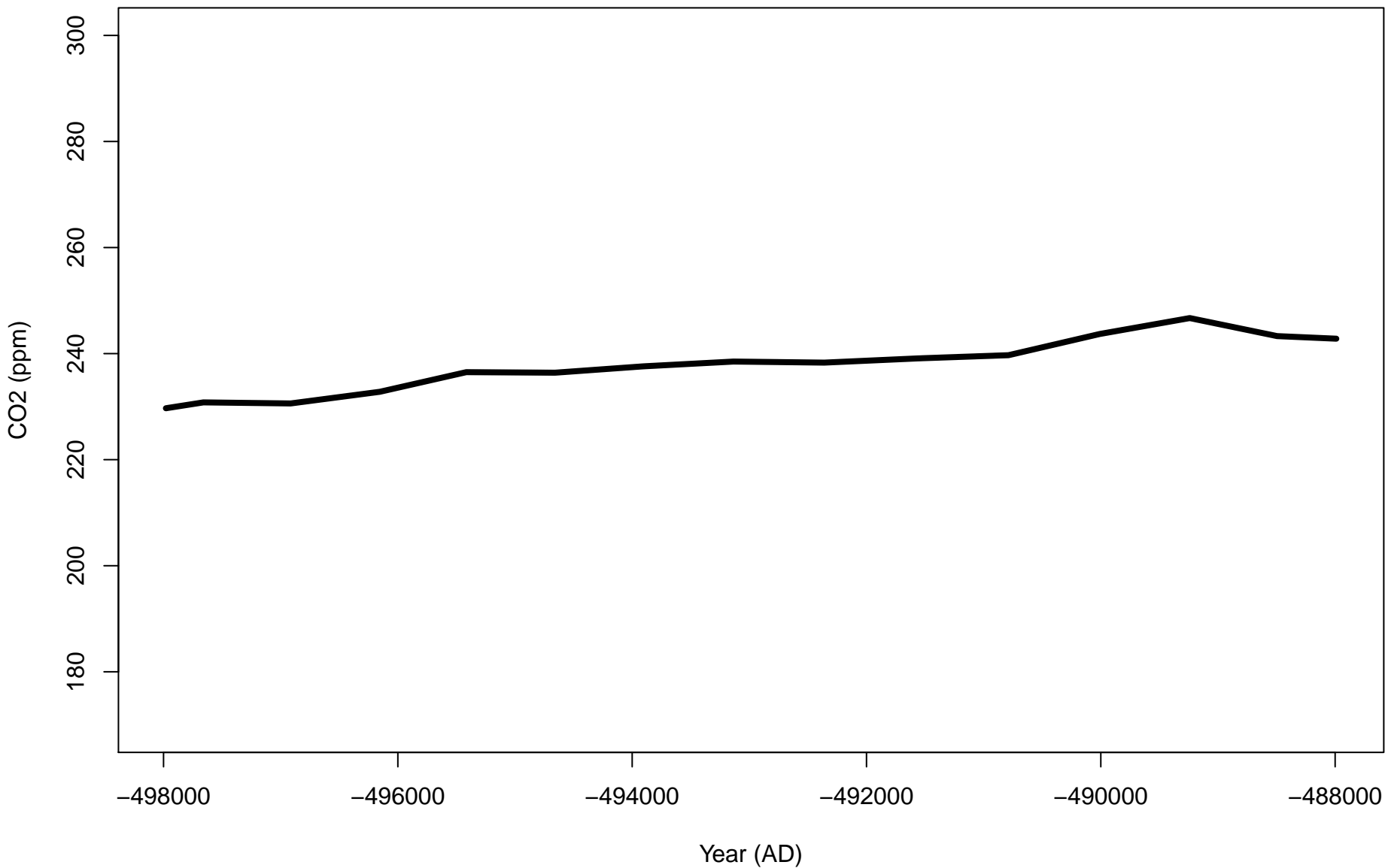
Past CO2 with 100 Centuries per Page
