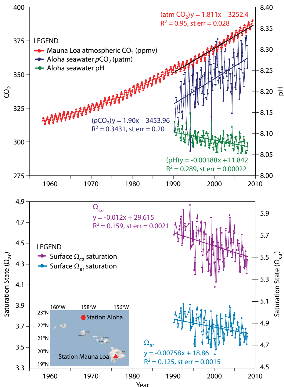
Figure 1. (Top) Time series of atmospheric \text{CO}_2 at Mauna Loa (ppmv) and surface ocean pH and p\text{CO}_2 ( \mu\text{atm} ) at Ocean Station Aloha in the subtropical North Pacific Ocean (see inset map). Note that the increase in oceanic \text{CO}_2 over the period of observations is consistent with the atmospheric increase within the statistical limits of the measurements. (Bottom) Calcite and aragonite saturation data for surface waters. Mauna Loa data: Pieter Tans, NOAA/ESRL, http://www.esrl.noaa.gov/gmd/ccgg/trends . HOT/ALOHA data: David Karl, University of Hawaii, http://hahana.soest.hawaii.edu . Updated from Doney et al. (2009). See also Dore et al. (2009).
