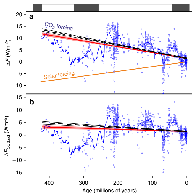
Figure 2 | Temporal evolution of climate forcing. (a) \text{CO}_2 data (blue circles) and LOESS best fit (blue line; Supplementary Data 2) with \Delta F for \text{CO}_2 calculated as in equation (6). The change in solar forcing ( \Delta F_{\text{sol}} ) calculated using equations (2 and 3). (b) \Delta F_{\text{CO}_2,\text{sol}} for data (blue circles) and LOESS best fit (blue line). Red line is a linear best fit and 95% confidence interval for least squares regression through the \Delta F_{\text{CO}_2,\text{sol}} data (blue circles; m = -0.004 \pm 0.001 1 s.e.m., R^2 = 0.01 , P = 0.0003 ). Black line is least squares fit through the LOESS best fit resampled to original data density (blue line; m = 0.008 \pm 0.001 1 s.e.m., R^2 = 0.06 , P < 0.0001 ). Icehouse time intervals are indicated by a black band and greenhouse intervals by a white band.
