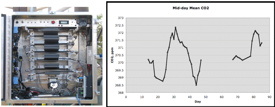
Figure 8. Precision carbon dioxide and flask sampling system (left) and midday atmospheric CO 2 concentration measurements (right) at the Skukuza eddy flux site in the Kruger National Park, South Africa. The system uses automatic calibration with WMO-traceable standards and a temperature controlled infrared gas analyzer to measure CO 2 concentration to an absolute precision of ~0.2 ppm.
