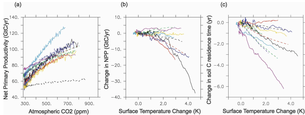
FIG. 3. (a) Simulated NPP sensitivity to atmospheric CO 2 (uncoupled run). (b) Simulated NPP sensitivity to climate (coupled run – uncoupled run). (c) Simulated soil carbon turnover time sensitivity to climate (coupled run – uncoupled run). Color code is the same as in Fig. 1.
