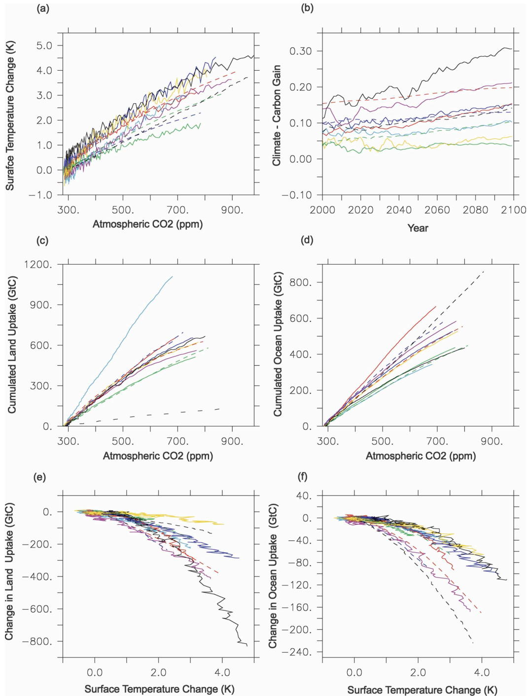
FIG. 2. (a) Simulated surface temperature response to atmospheric CO 2 . (b) Time evolution of the climate-carbon gain. (c) Sensitivity of land carbon storage to atmospheric CO 2 (uncoupled runs). (d) Same as (c) for the ocean. (e) Sensitivity of land carbon storage to climate (coupled runs). (f) Same as (e) for the ocean. Color code is the same as in Fig. 1.
