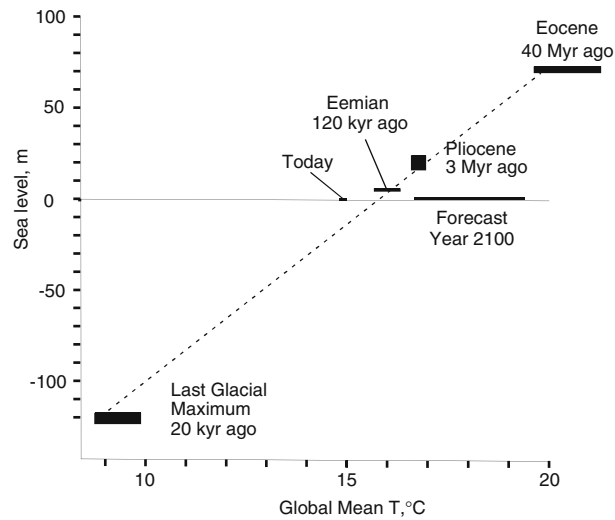
Fig. 3 The relationship between sea level and temperature on geologic time scales. Data from (Alley et al. 2005)
